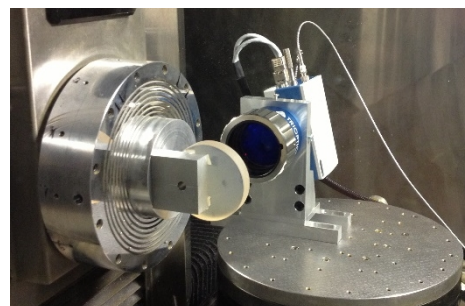
Customized mounted \mu Phase ® base module for measuring inside a manufacturing machine
